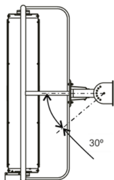
Side view, 30° vertical adjustment
