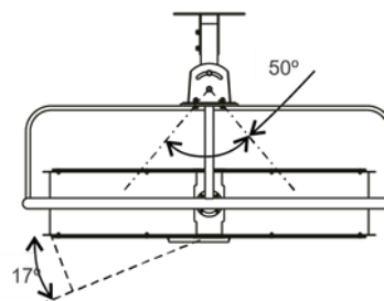
Floor view, 34° pivoting option and 50° horizontal adjustment
